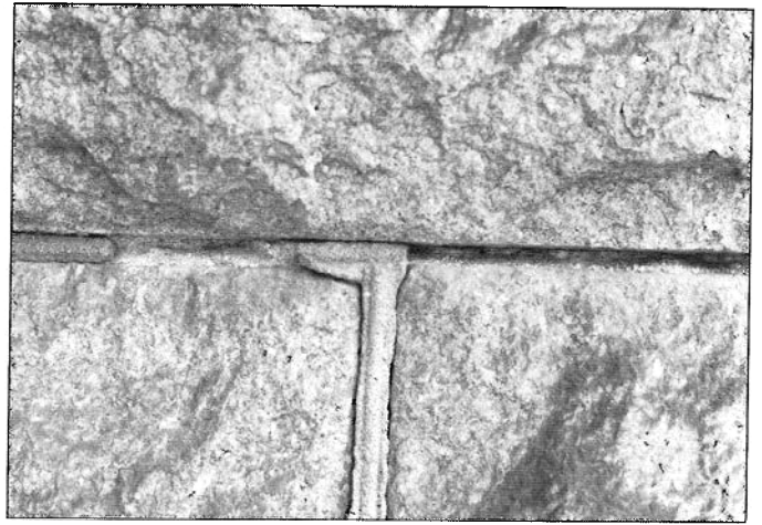
Figure 8. Due to inadequate joint preparation, the repointing mortar has not adhered properly and is falling out of the joint. Photo: Robert C. Mack, FAIA.
