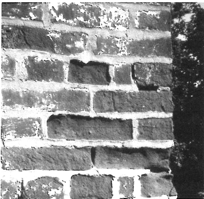
Figure 5. The use of hard, portland-cement mortar that is less permeable than the soft bricks has resulted in severe damage to this brick wall. Moisture trapped in the wall was unable to evaporate through the mortar which is intended to be sacrificial, and thus protect the bricks. As a result the moisture remained in the walls until water pressure eventually popped the surface off the bricks. Photo: National Park Service Files.
