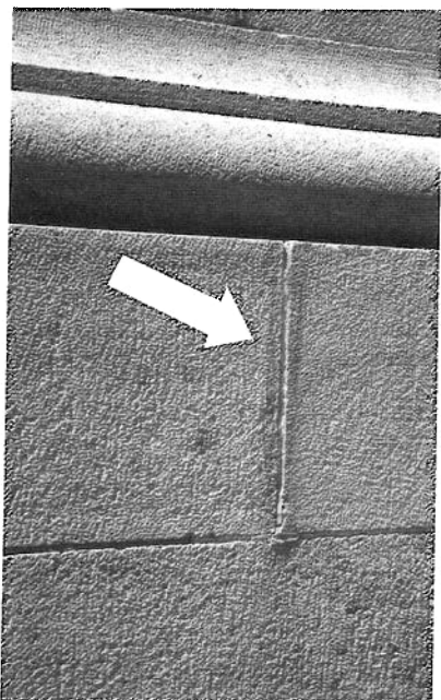
Figure 7. The dark stain on either side of the vertical joint on this sandstone water table probably resulted from the use of a bonding agent that was not properly cleaned off the masonry after repointing. Photo: Anne Grimmer.
