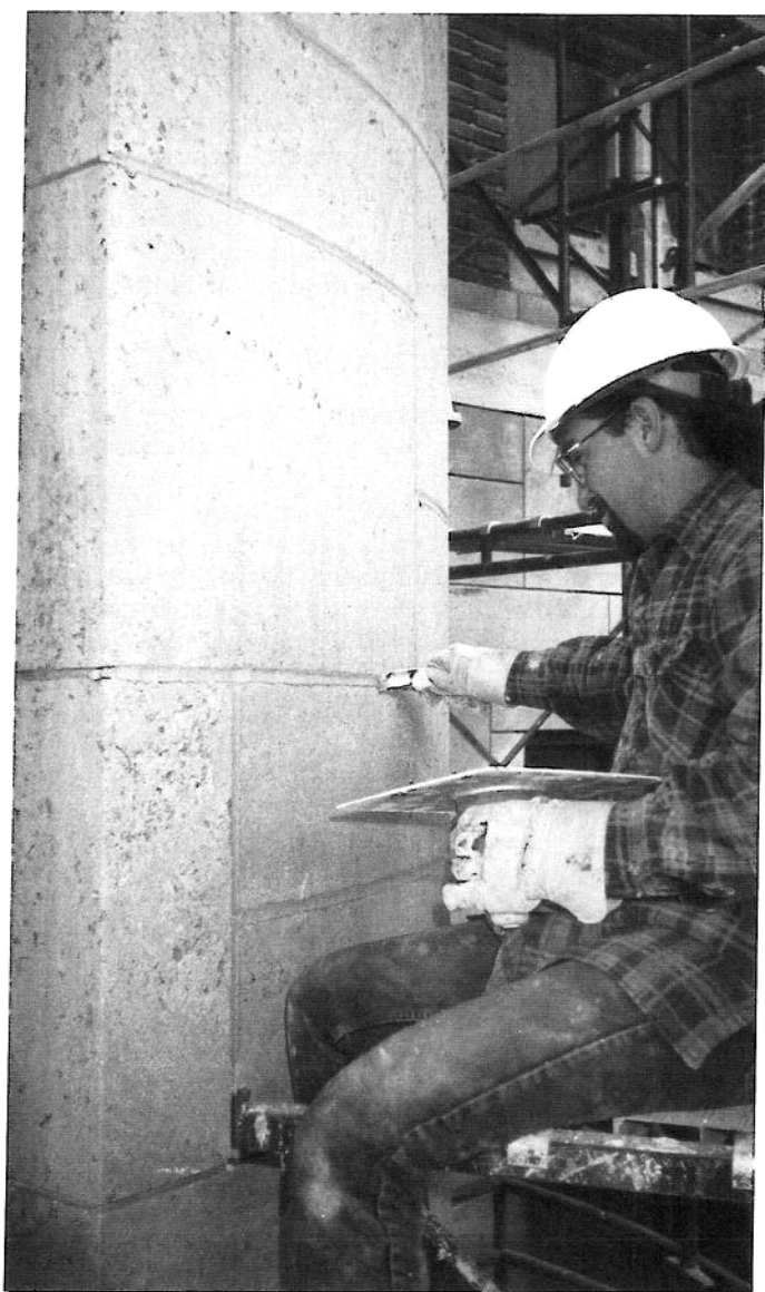
Figure 1. After removing deteriorated mortar, an experienced mason repoints a portion of this early-20th century limestone building. Photo: Robert C. Mack, FAIA.
